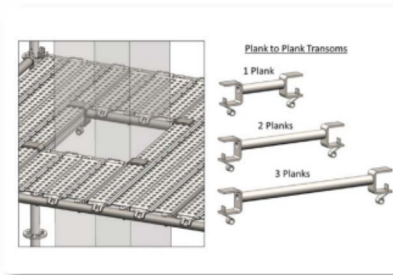
Plank to plank
