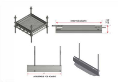
Adjustable toe boards
