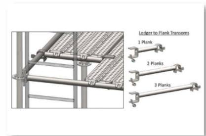
Ledger to plank
